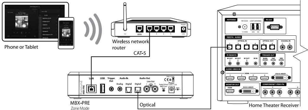
Connection with home theater receiver
