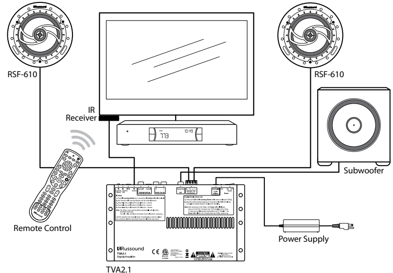
Typical TVA2.1 Amplifier Installation
