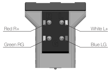
Cartridge back view
